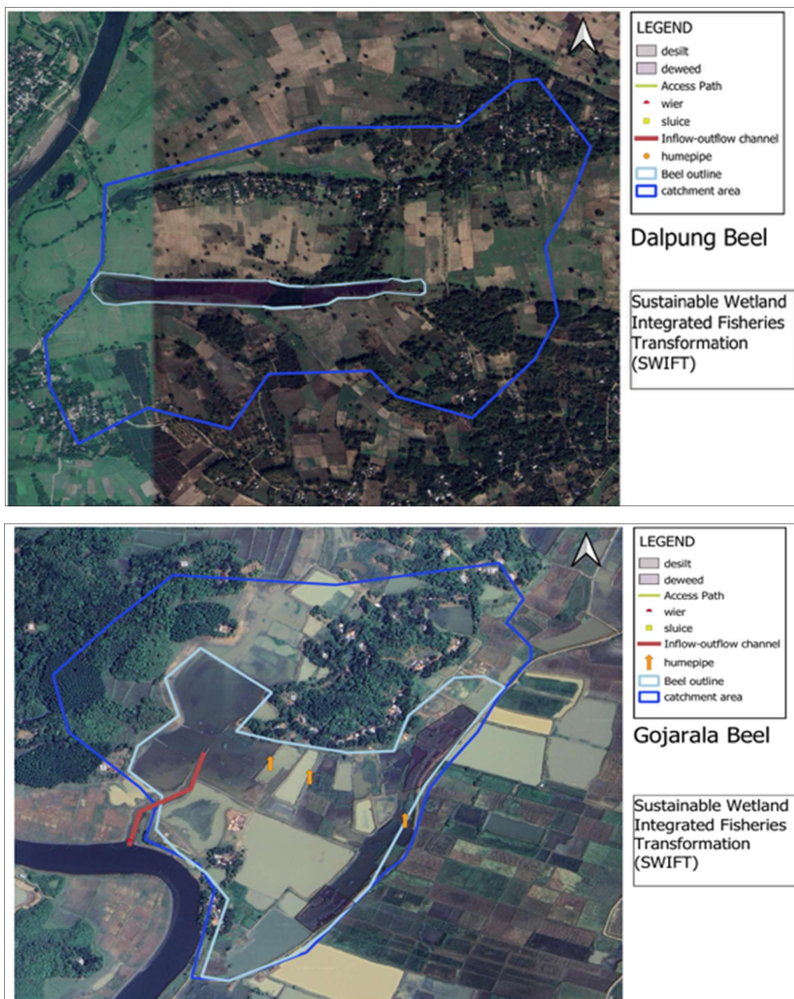
Figure 3-7. Layout catchment of Dalpung and Gojarala Beels including possible sites for proposed interventions
