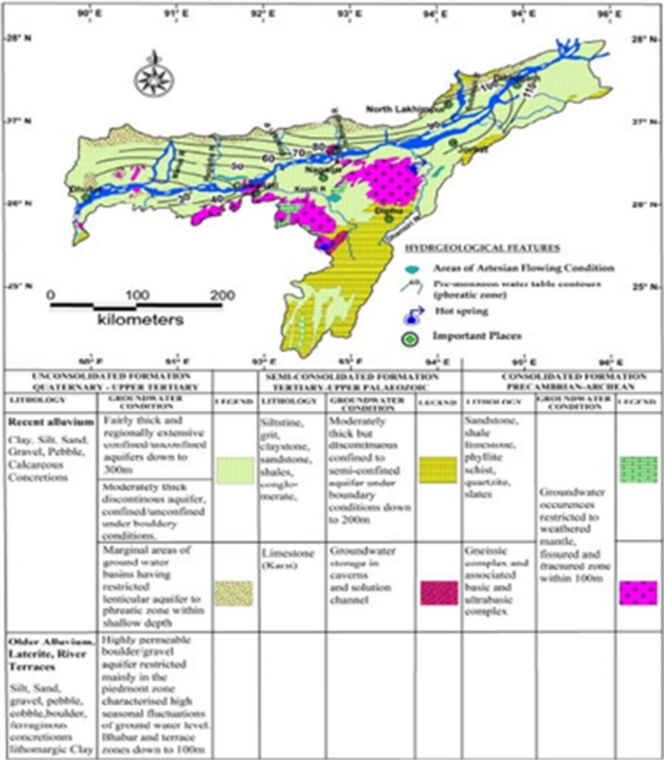
Figure 4-5. Hydrogeological Map of Assam 35
