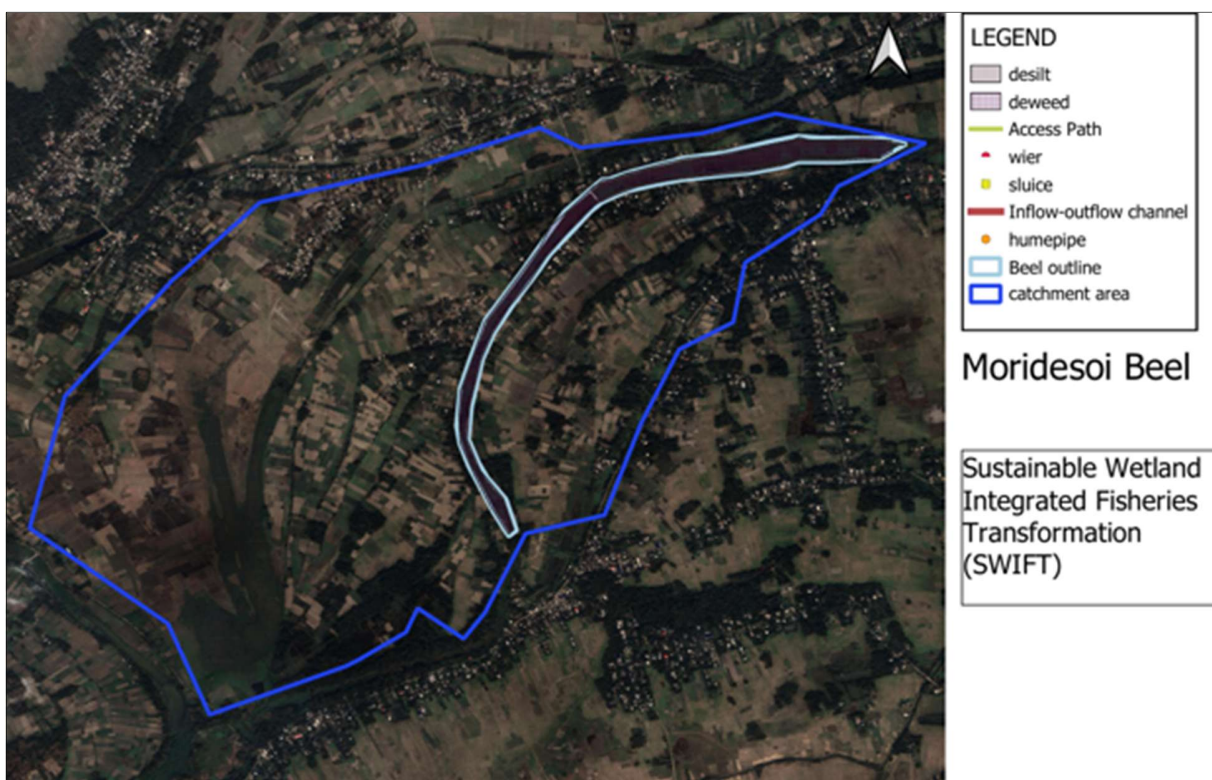
Figure 3-8. Layout catchment of Mahara Anchalikg and Moridesoi Beel including possible sites for proposed interventions
