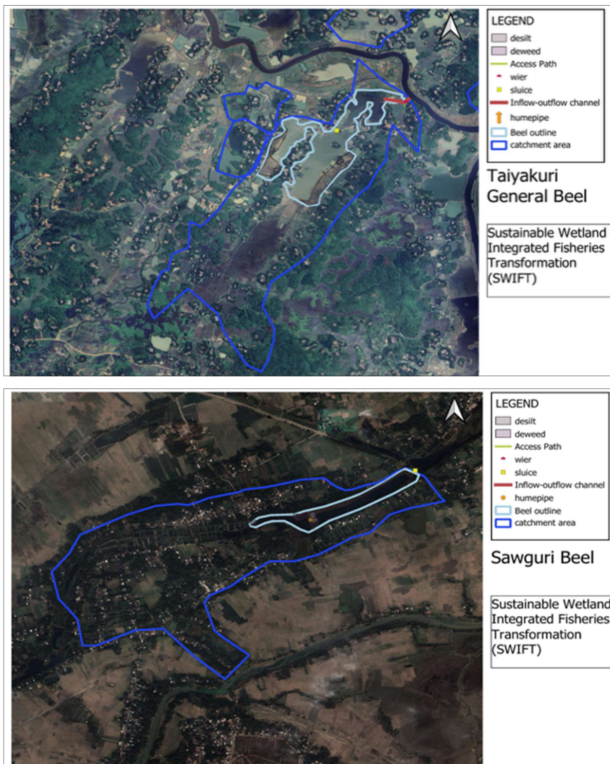
Figure 3-10. Layout catchment of Taiyakauri and Sawguri Beels including possible sites for proposed interventions
