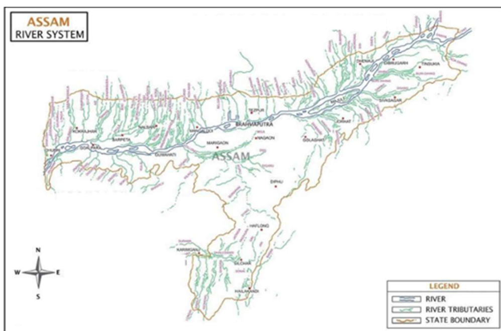
Figure 4-4. River System map of Assam (Source: DPR)
