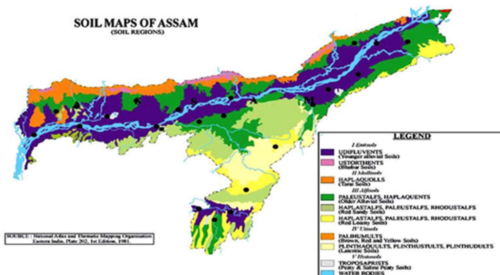
Figure 4-6. Soil Regions of Assam 37
