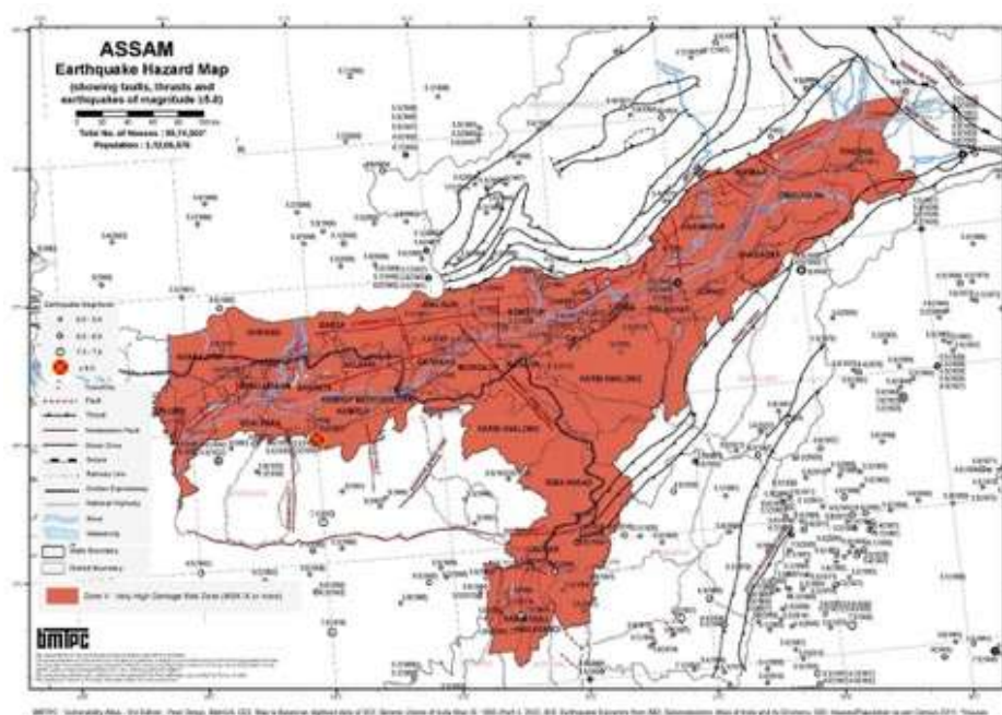
Figure 4-8. Earthquake Hazard Map of Assam 39
