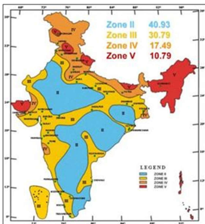
Figure 4-7. Seismic Zonation Map of India 38
