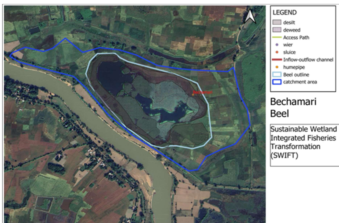
Figure 3-5. Layout of Bechamari beel catchment and possible sites for proposed interventions
