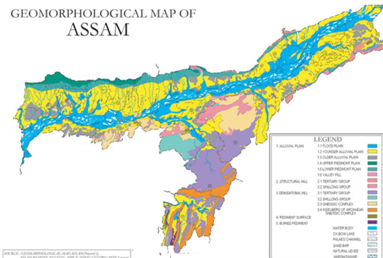
Figure 4-3. Geomorphological Map of Assam
